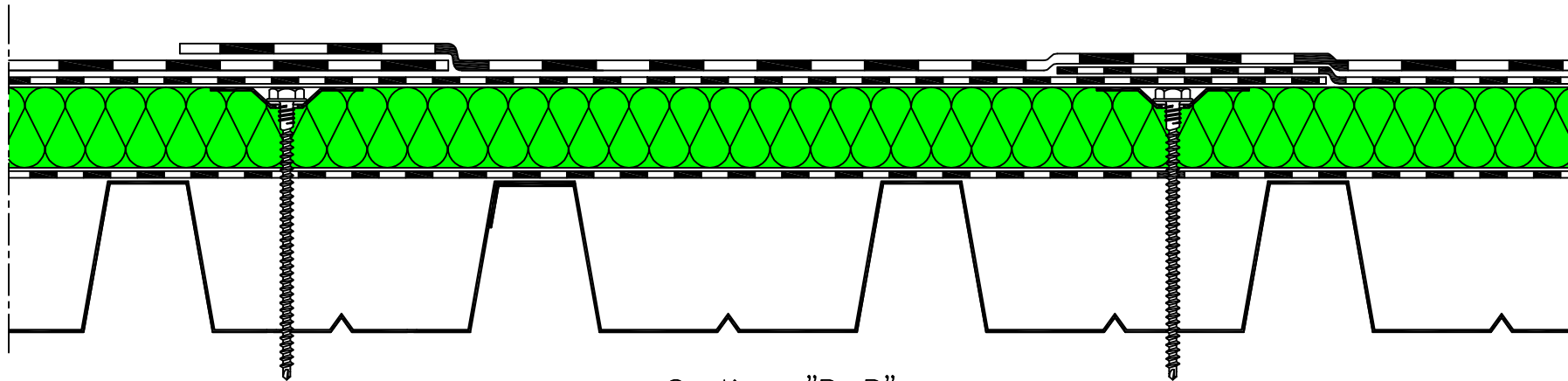
Section: "B-B"
