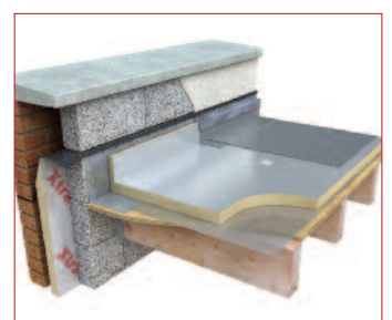
Typical installation - Timber Deck
