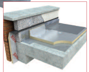
Typical installation - Concrete Deck
